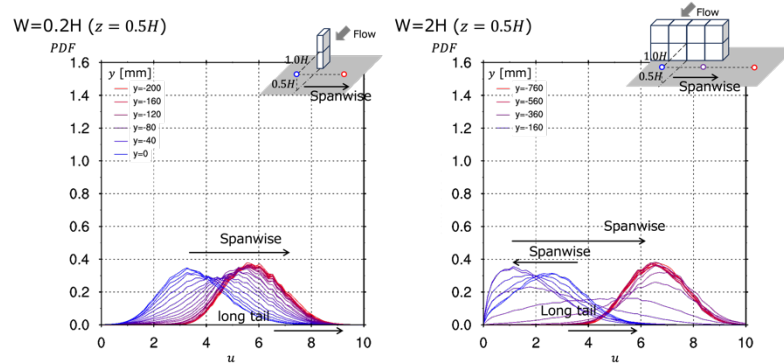
Fig.1 Probability density distributions of the wind speed within the wake of two types of blocks with the width of 0.2H and 2H at different spanwise locations.
